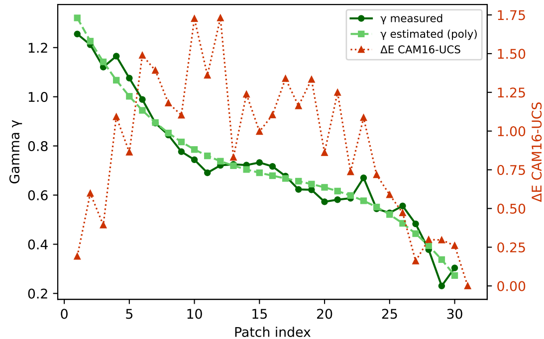
G — gamma (degree 3) mean \Delta E=0.898 std=0.468
