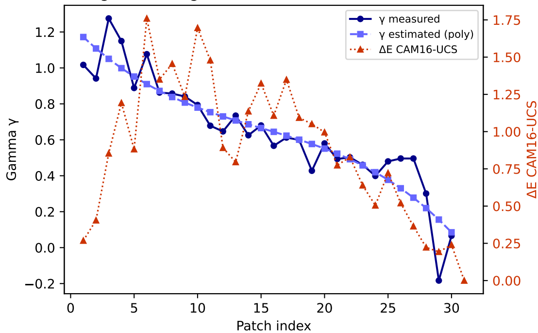
B — gamma (degree 3) mean \Delta E=0.882 std=0.459
